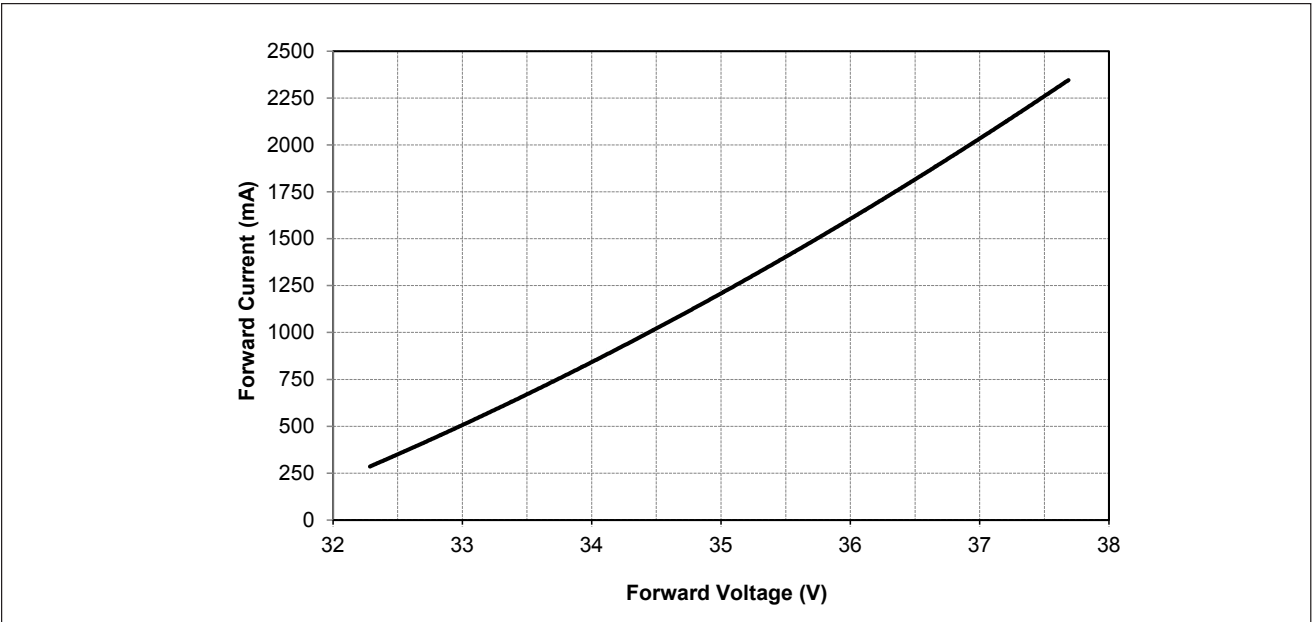
Figure 2: V18C Drive Current vs. Voltage ( T_j = T_c = 25^\circ\text{C} )
