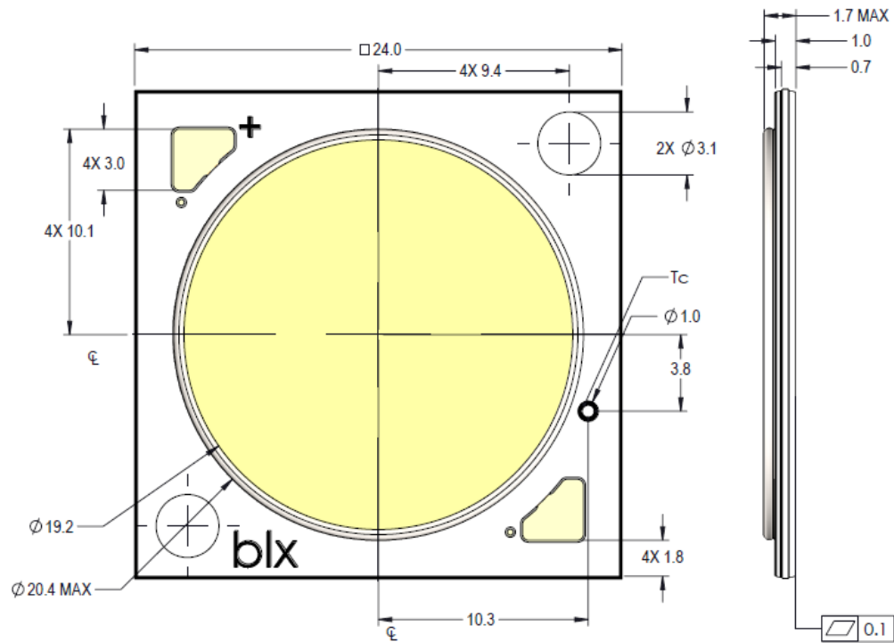
Figure 11: V18 LED Array
