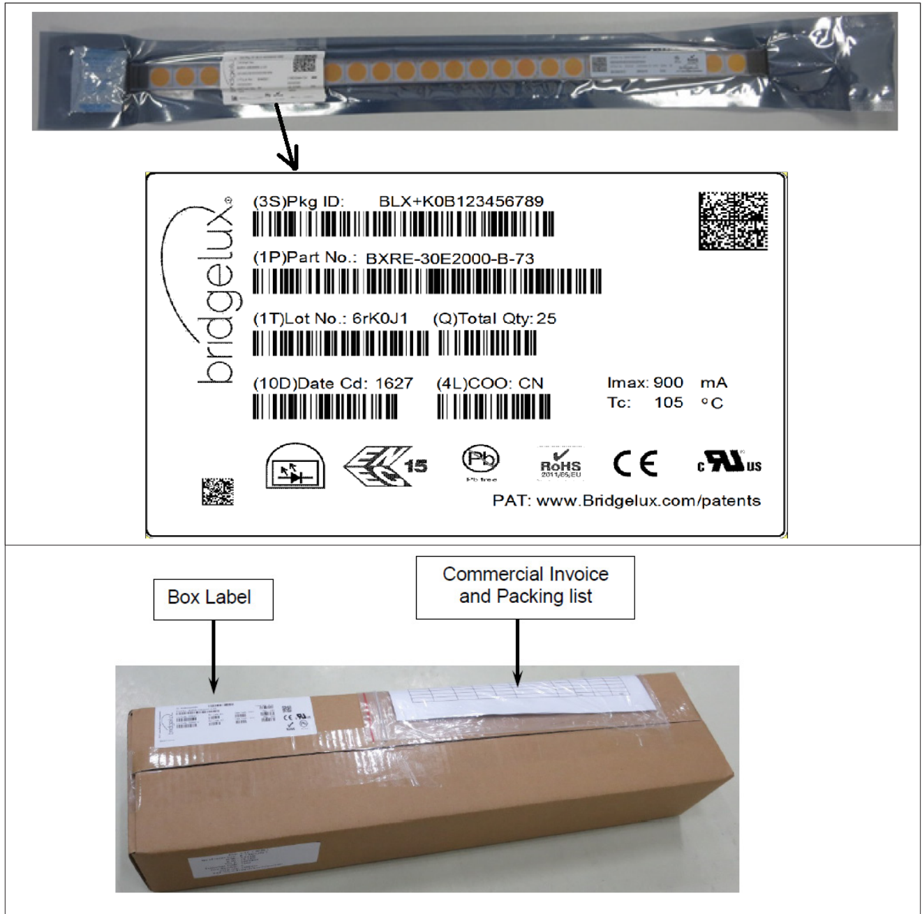
Figure 14: Drawing for V18 Packaging Tube
