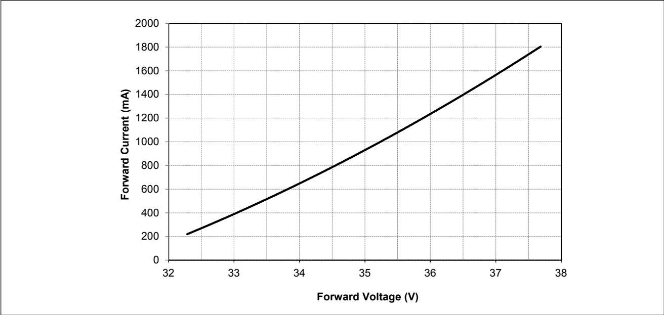
Figure 1: V18B Drive Current vs. Voltage ( T_j = T_c = 25^\circ\text{C} )
