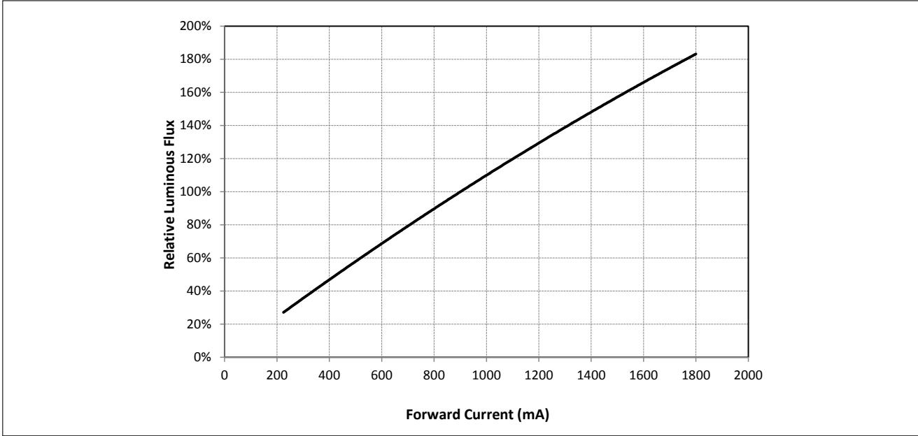
Figure 3: V18B Typical Relative Flux vs. Current ( T_j = T_c = 25^\circ\text{C} )
