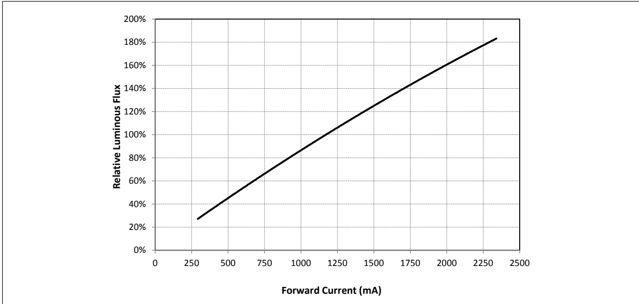
Figure 4: V18C Typical Relative Flux vs. Current ( T_j = T_c = 25^\circ\text{C} )
